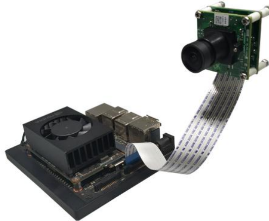
Fig-1: e-CAM50_CUNX - 5MP MIPI camera for NVIDIA® Jetson Xavier NX™ Developer Kit
